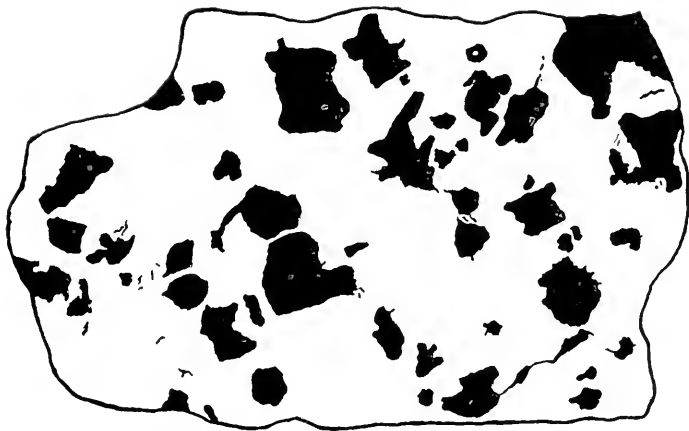
Fig. 62—"Spotted" diorite, actual size, Frood ore body, Sudbury area, Ontario. Black represents sulphides; white represents diorite. The sulphides replace or impregnate the rock.
